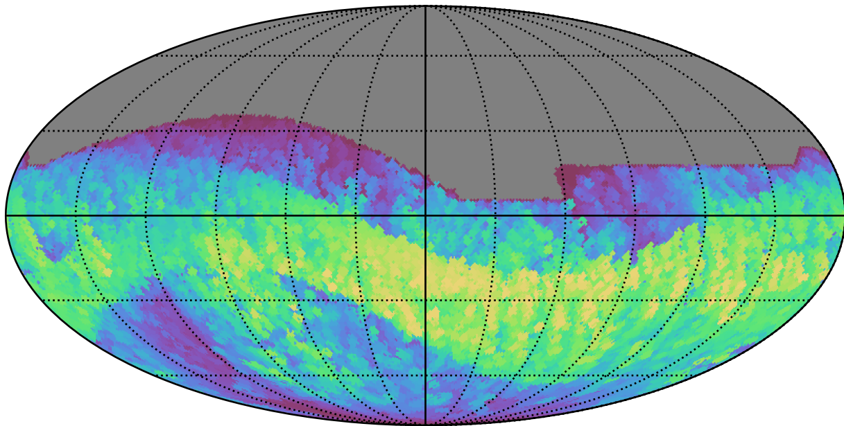
too_10_1v3.4_10yrs All sky z band: Max normairmass
