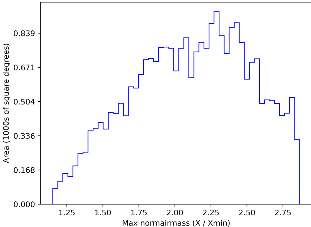
too_10_1v3.4_10yrs All sky z band: Max normairmass
