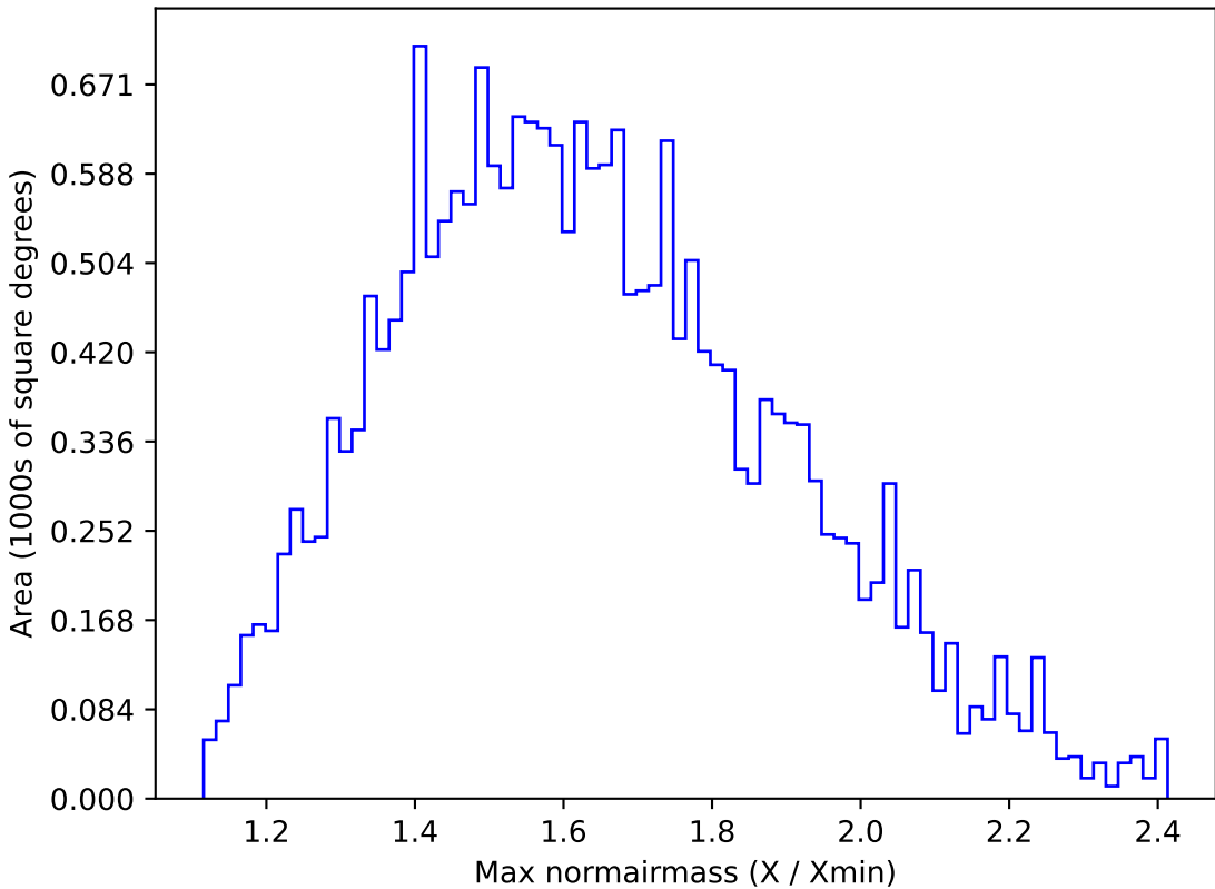
too_10_1v3.4_10yrs All sky u band: Max normairmass
