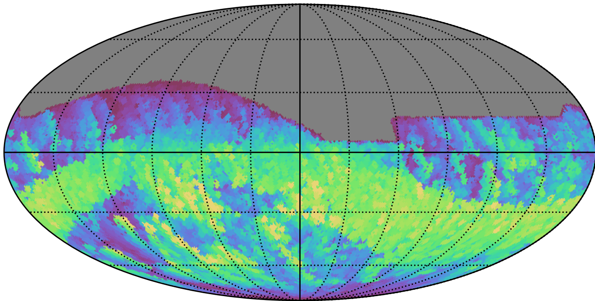
too_10_1v3.4_10yrs All sky r band: Max normairmass
