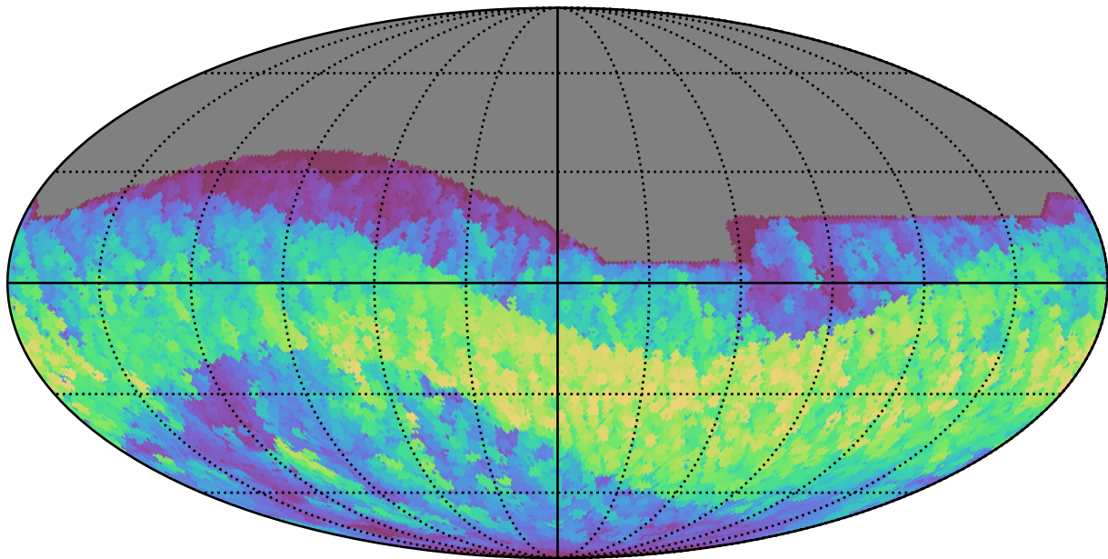
too_10_1v3.4_10yrs All sky i band: Max normairmass
