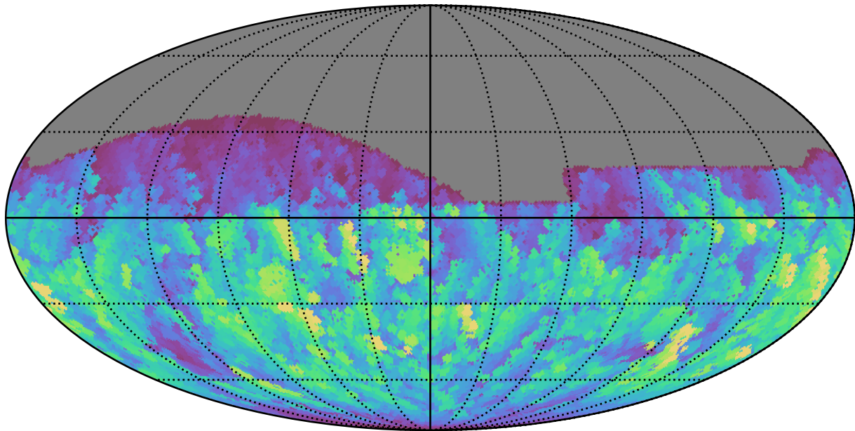
too_10_1v3.4_10yrs All sky g band: Max normairmass
