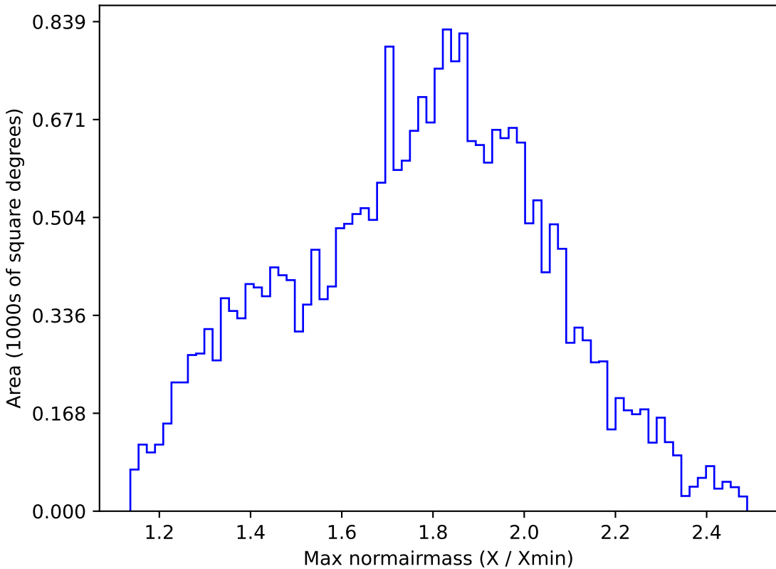
too_10_1v3.4_10yrs All sky g band: Max normairmass
