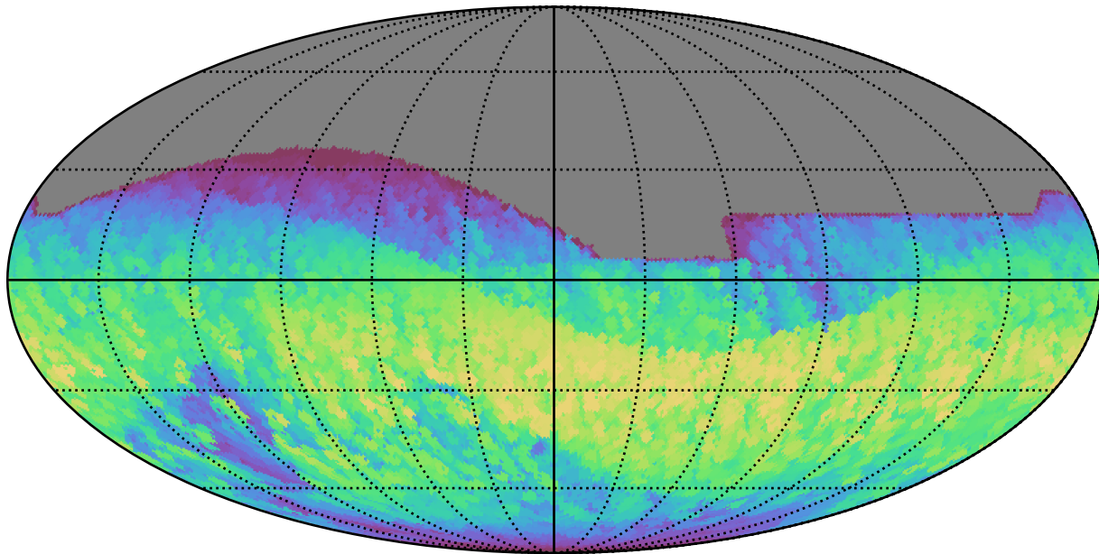
too_10_1v3.4_10yrs All sky all bands: Max normairmass
