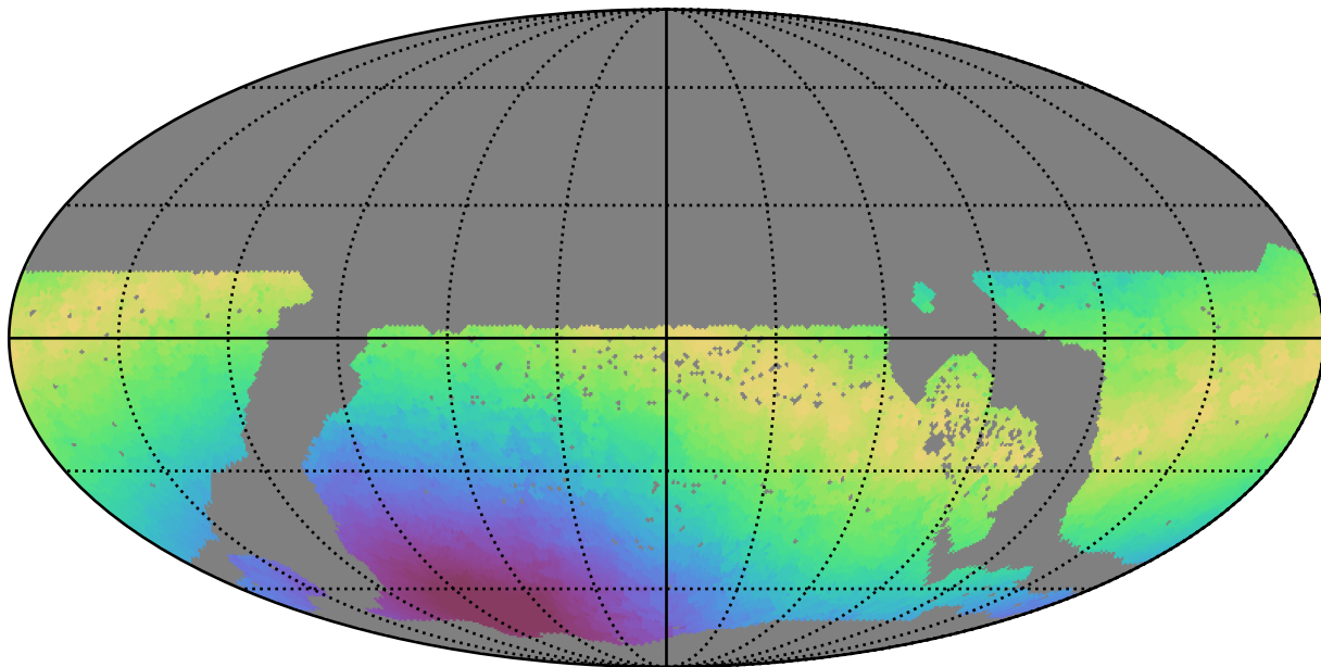
too_10_1v3.4_10yrs WFD z band: Max moonDistance
