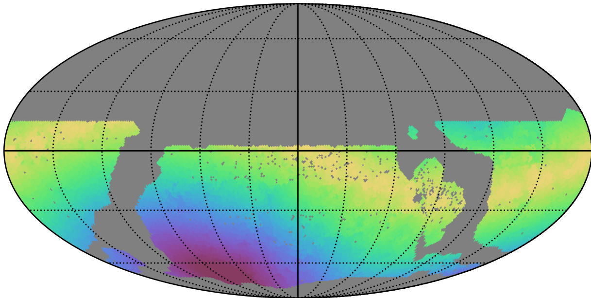
too_10_1v3.4_10yrs WFD u band: Max moonDistance
