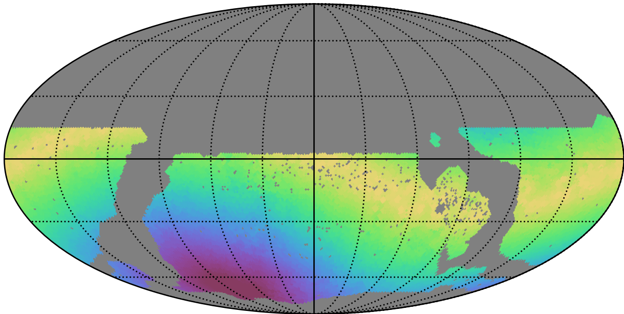
too_10_1v3.4_10yrs WFD i band: Max moonDistance
