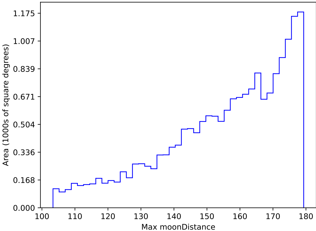
too_10_1v3.4_10yrs WFD i band: Max moonDistance
