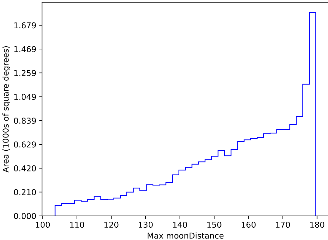
too_10_1v3.4_10yrs WFD all bands: Max moonDistance
