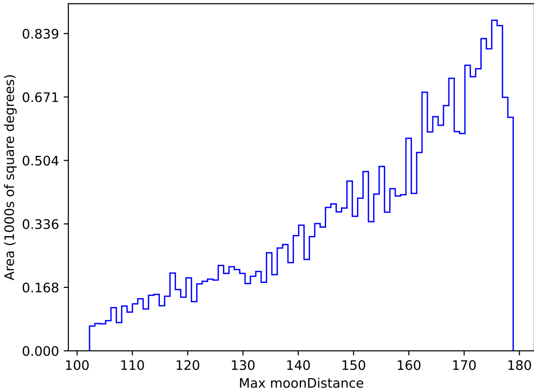
too_10_1v3.4_10yrs All sky z band: Max moonDistance
