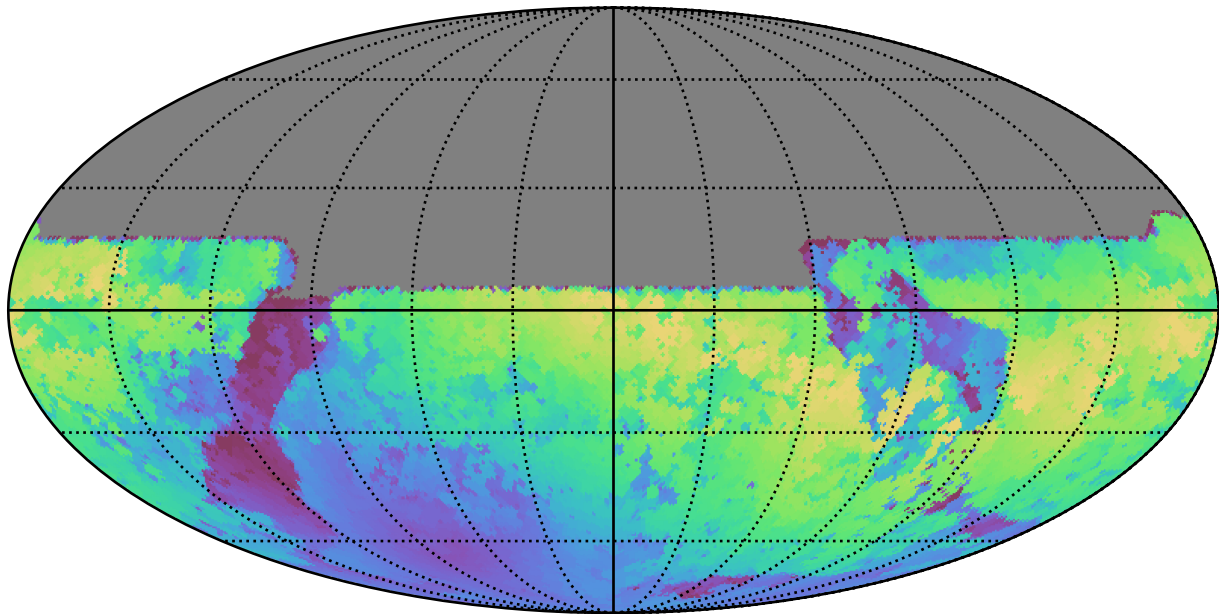
too_10_1v3.4_10yrs All sky y band: Max moonDistance
