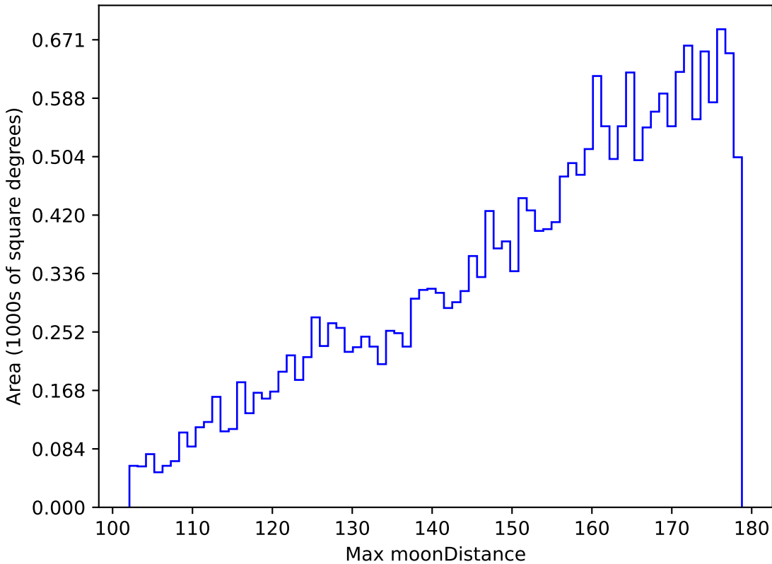
too_10_1v3.4_10yrs All sky u band: Max moonDistance
