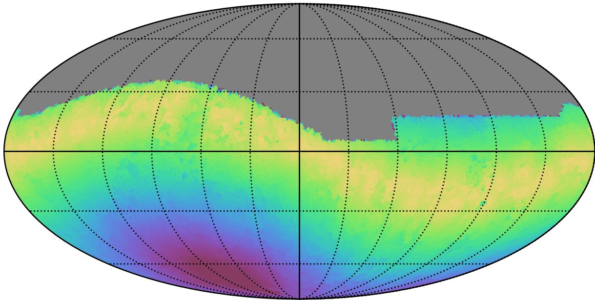
too_10_1v3.4_10yrs All sky g band: Max moonDistance
