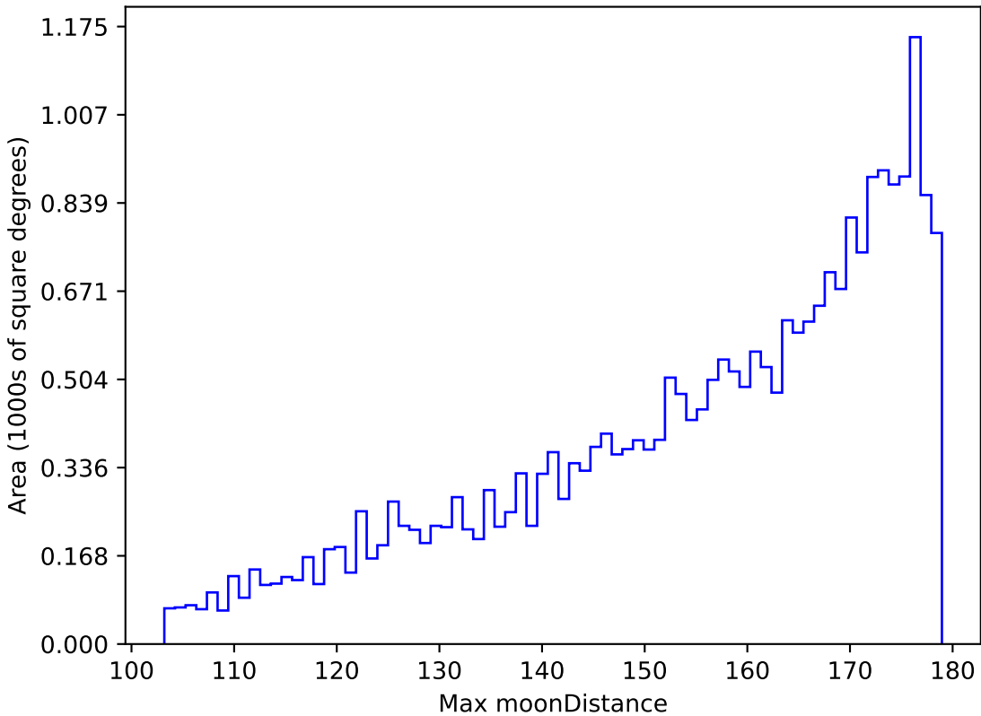
too_10_1v3.4_10yrs All sky g band: Max moonDistance
