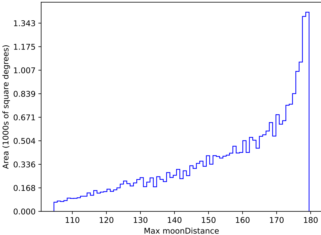
too_10_1v3.4_10yrs All sky all bands: Max moonDistance
