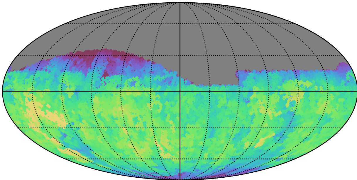
too_10_1v3.4_10yrs Yr 1 z band: Max fiveSigmaDepth
