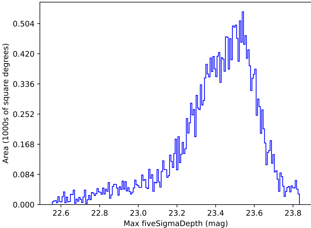
too_10_1v3.4_10yrs Yr 1 z band: Max fiveSigmaDepth
