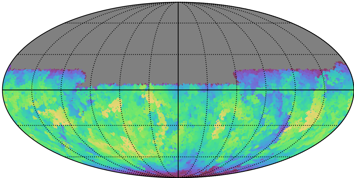
too_10_1v3.4_10yrs Yr 1 y band: Max fiveSigmaDepth
