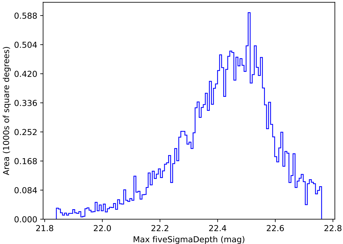
too_10_1v3.4_10yrs Yr 1 y band: Max fiveSigmaDepth
