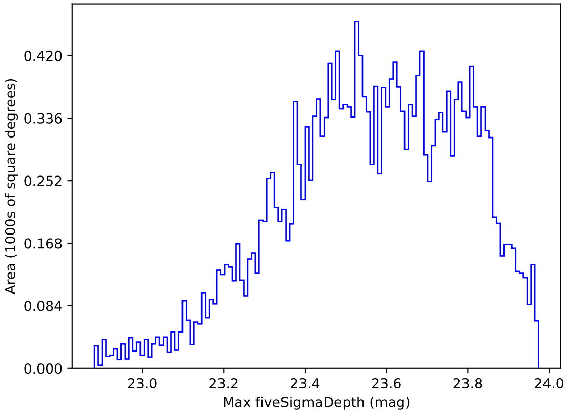
too_10_1v3.4_10yrs Yr 1 u band: Max fiveSigmaDepth
