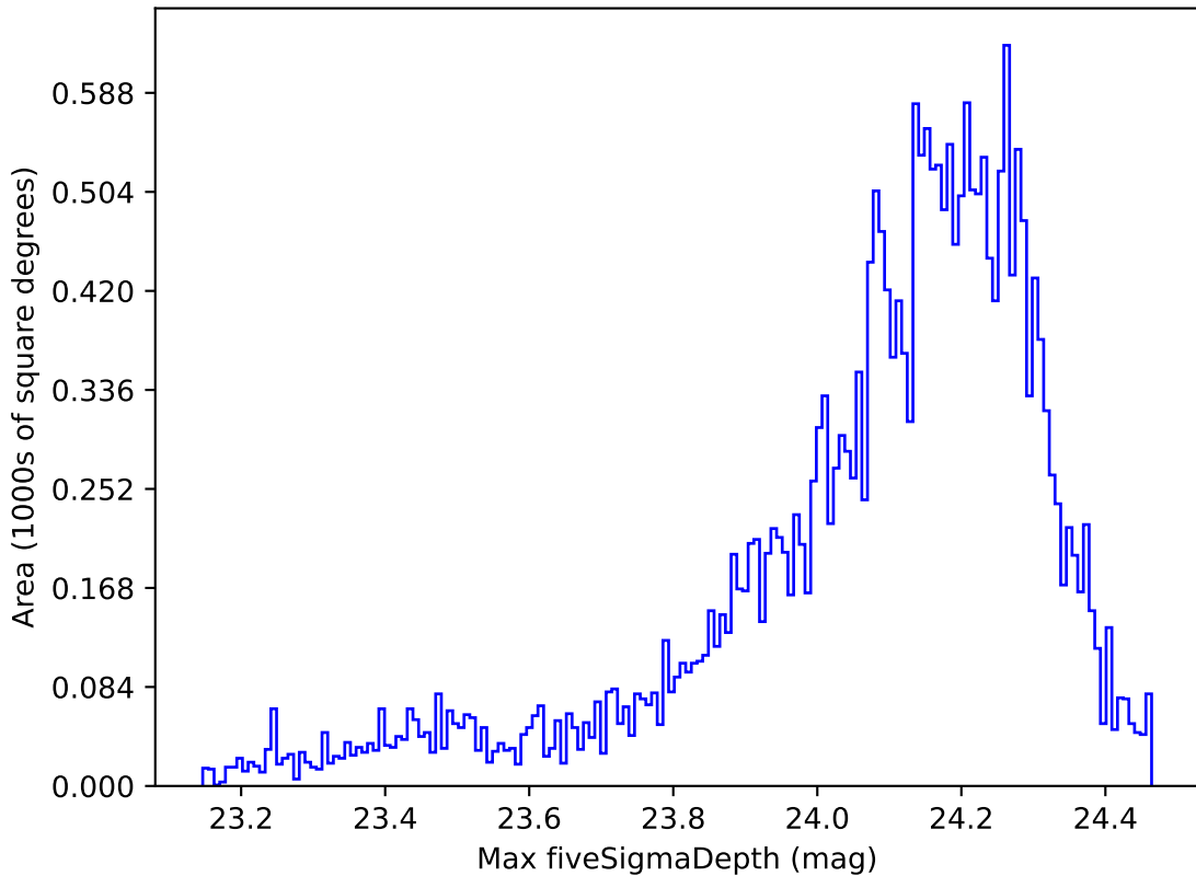
too_10_1v3.4_10yrs Yr 1 i band: Max fiveSigmaDepth
