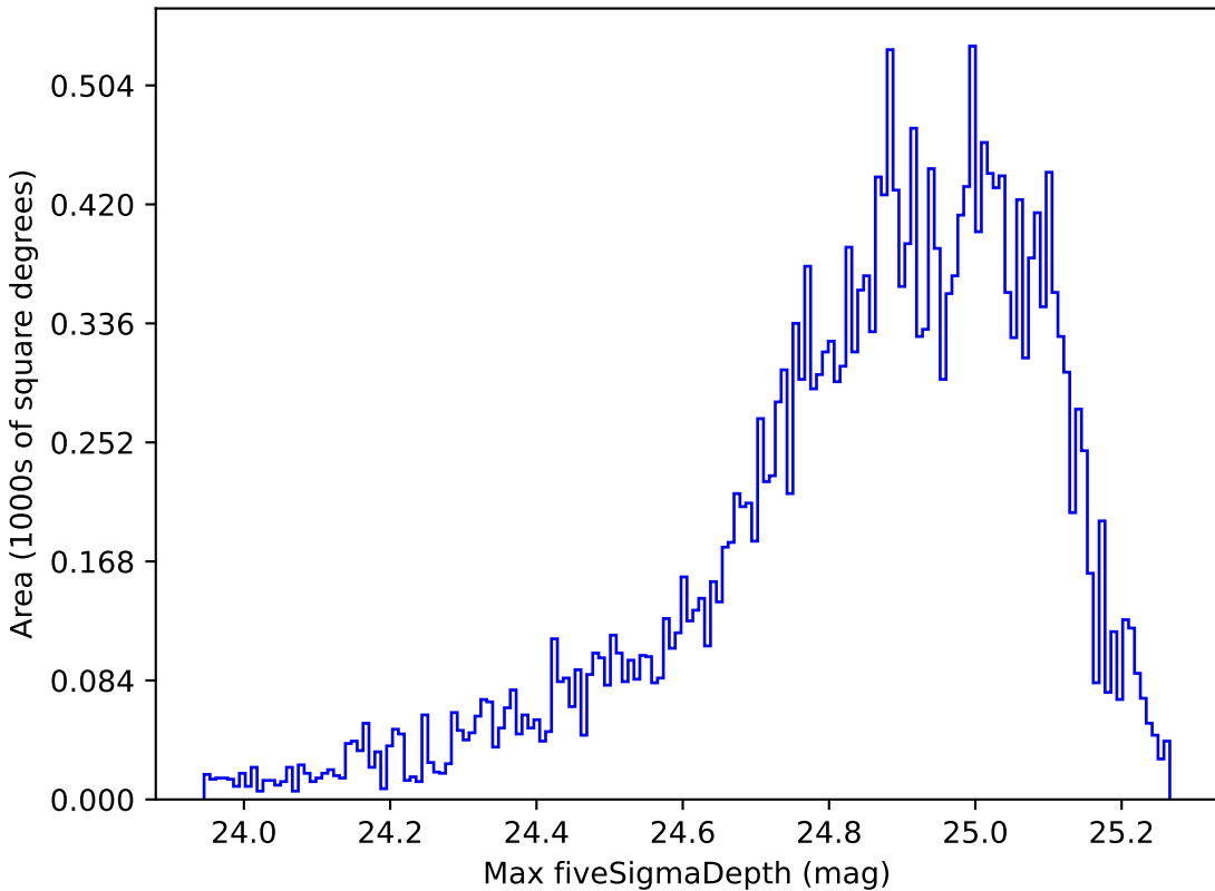
too_10_1v3.4_10yrs Yr 1 g band: Max fiveSigmaDepth
