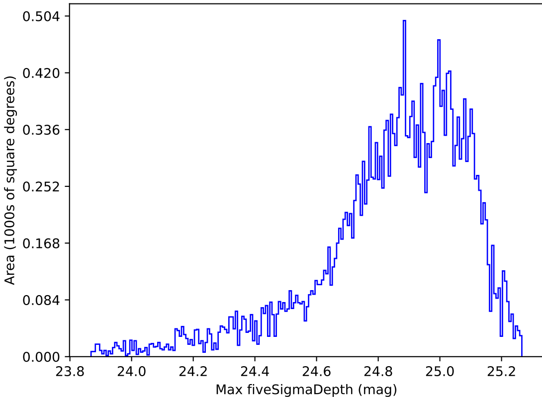
too_10_1v3.4_10yrs Yr 1 all bands: Max fiveSigmaDepth
