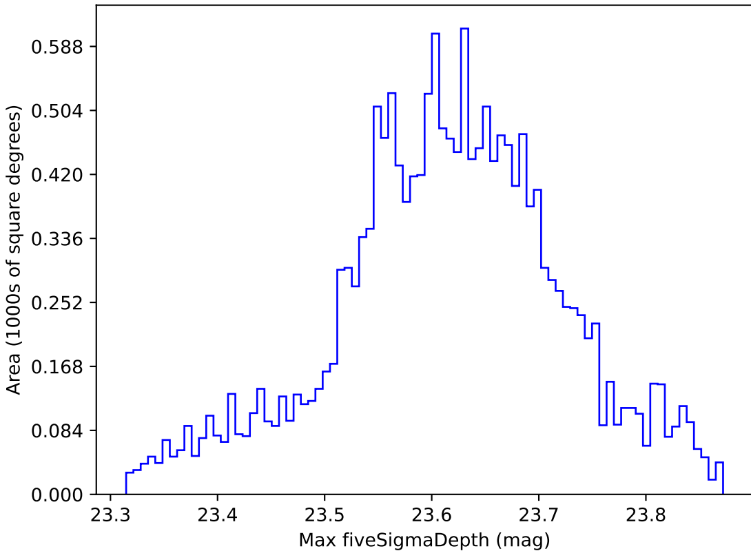
too_10_1v3.4_10yrs WFD z band: Max fiveSigmaDepth
