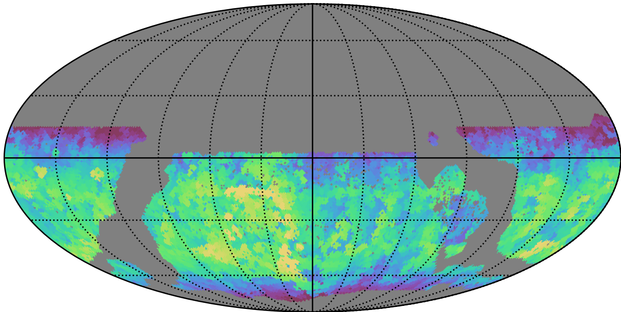
too_10_1v3.4_10yrs WFD y band: Max fiveSigmaDepth
