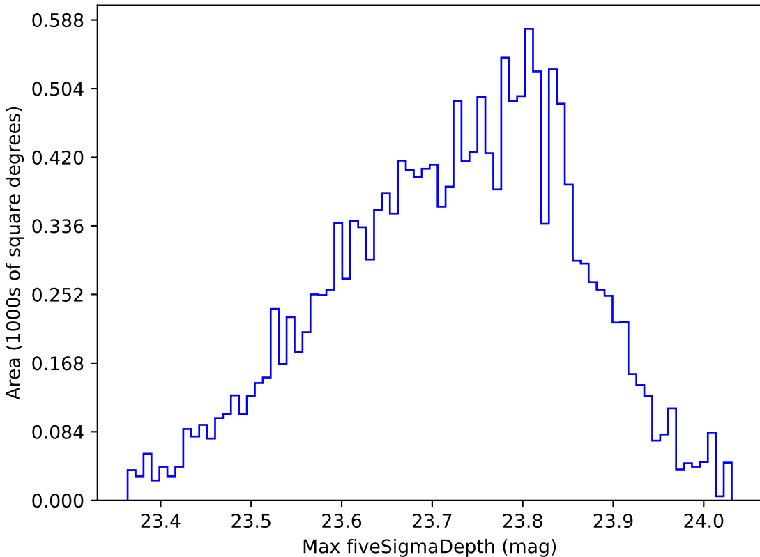
too_10_1v3.4_10yrs WFD u band: Max fiveSigmaDepth
