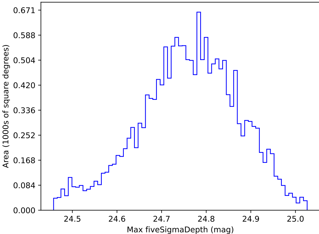
too_10_1v3.4_10yrs WFD r band: Max fiveSigmaDepth
