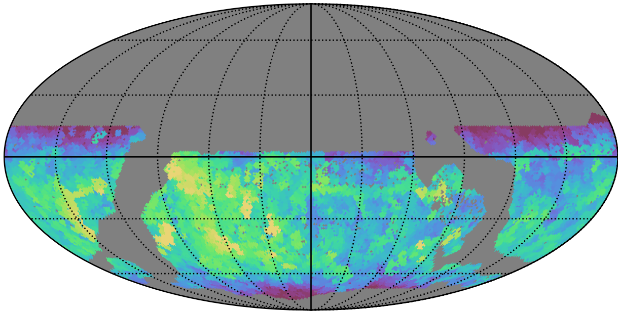
too_10_1v3.4_10yrs WFD i band: Max fiveSigmaDepth
