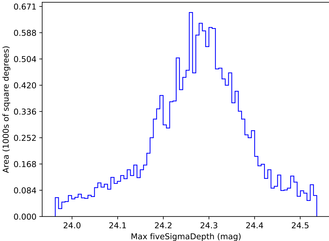
too_10_1v3.4_10yrs WFD i band: Max fiveSigmaDepth
