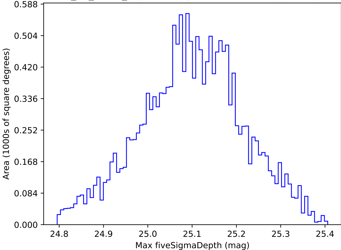
too_10_1v3.4_10yrs WFD g band: Max fiveSigmaDepth
