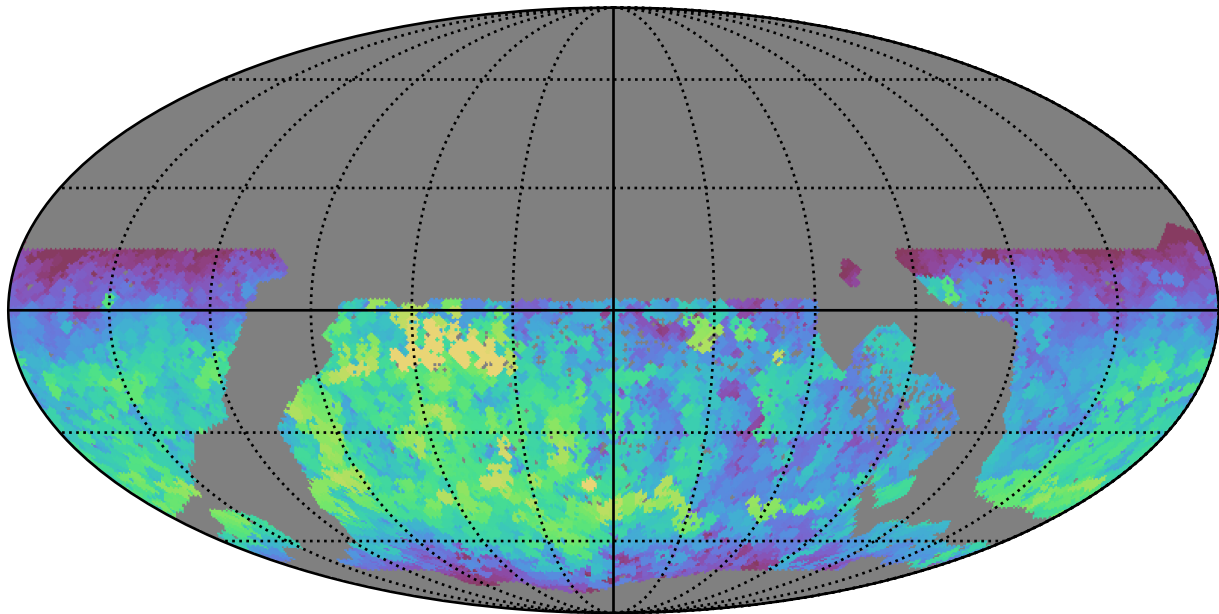
too_10_1v3.4_10yrs WFD all bands: Max fiveSigmaDepth
