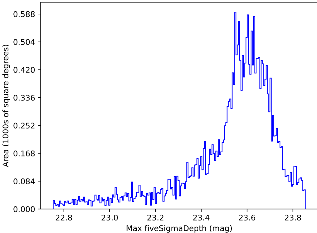
too_10_1v3.4_10yrs All sky z band: Max fiveSigmaDepth
