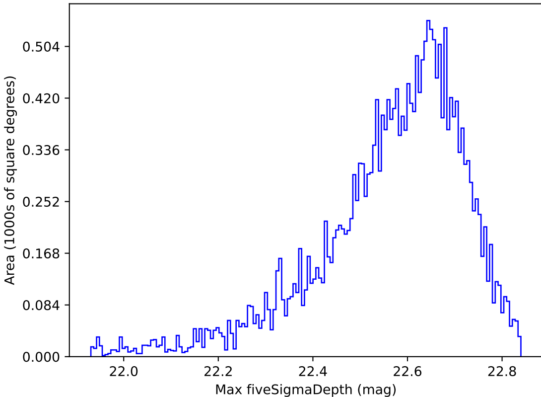
too_10_1v3.4_10yrs All sky y band: Max fiveSigmaDepth
