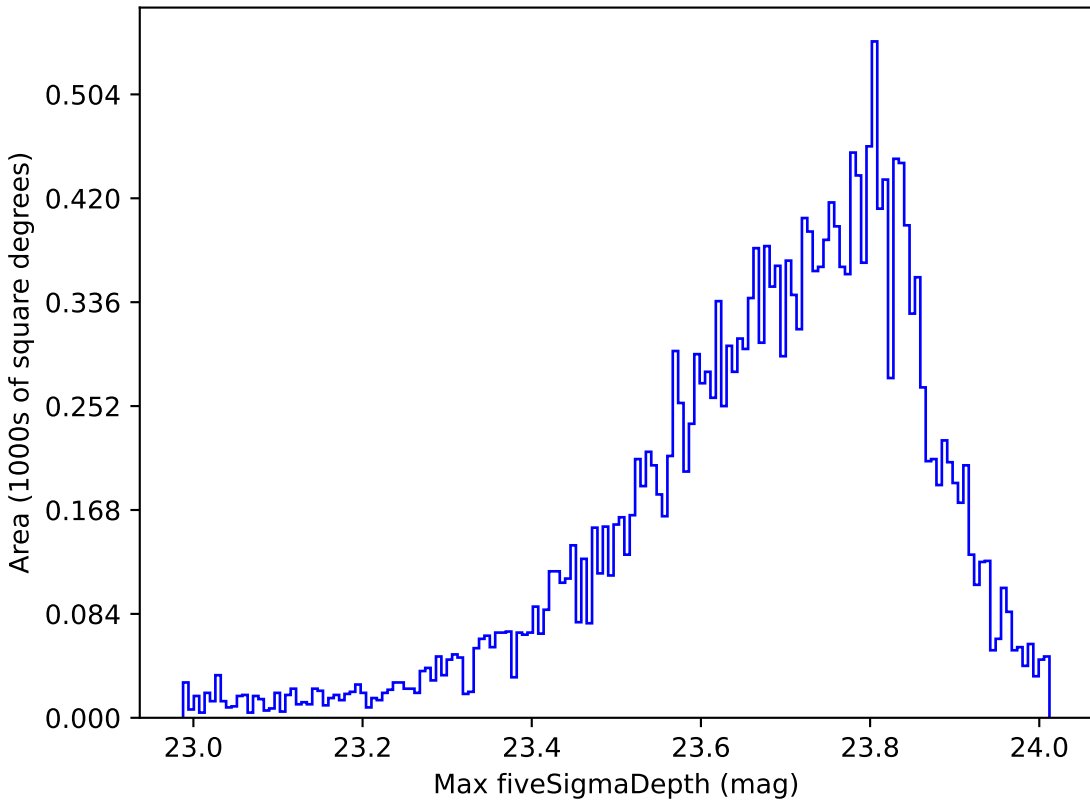
too_10_1v3.4_10yrs All sky u band: Max fiveSigmaDepth
