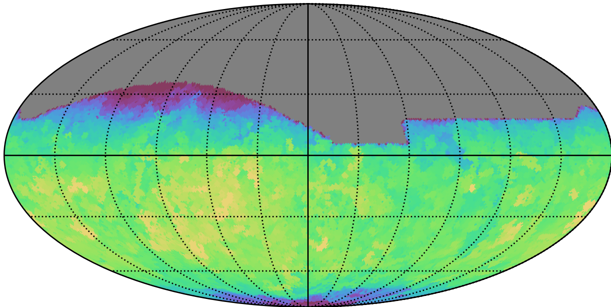
too_10_1v3.4_10yrs All sky r band: Max fiveSigmaDepth
