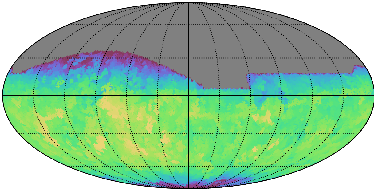
too_10_1v3.4_10yrs All sky i band: Max fiveSigmaDepth
