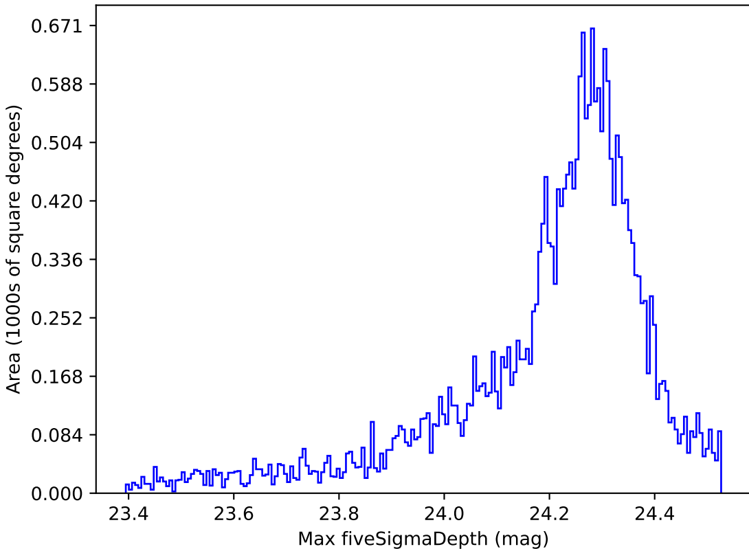
too_10_1v3.4_10yrs All sky i band: Max fiveSigmaDepth
