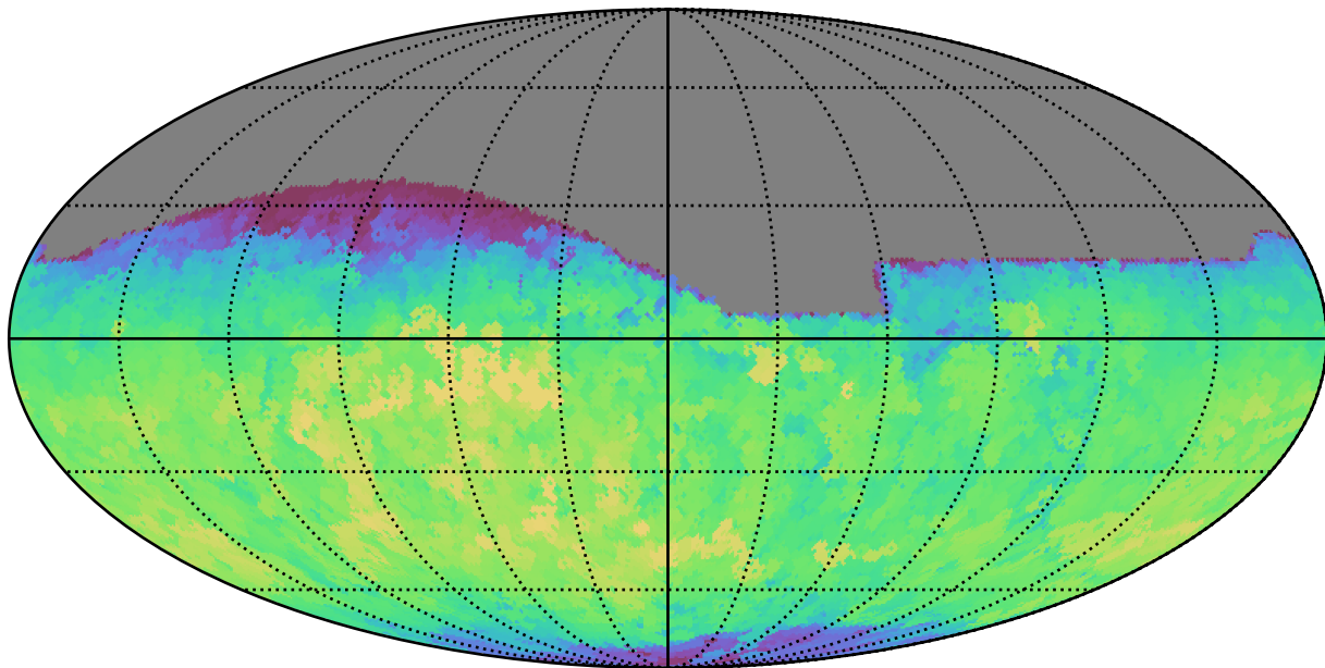
too_10_1v3.4_10yrs All sky g band: Max fiveSigmaDepth
