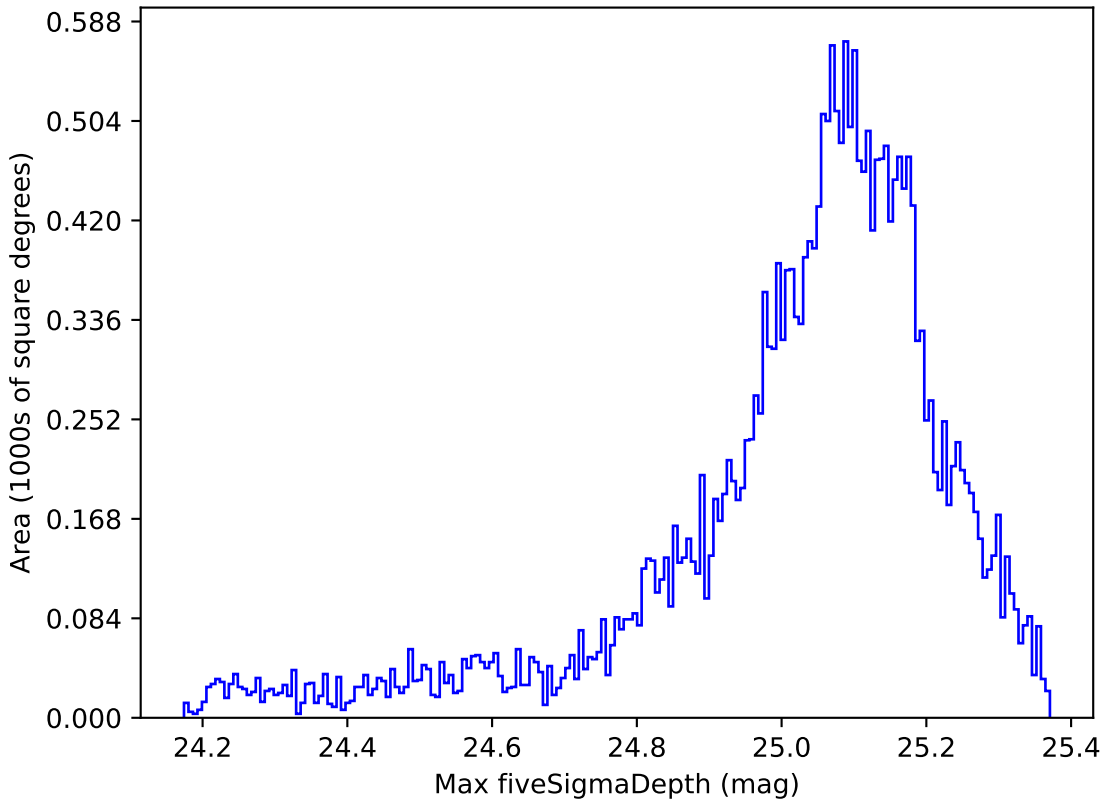
too_10_1v3.4_10yrs All sky g band: Max fiveSigmaDepth
