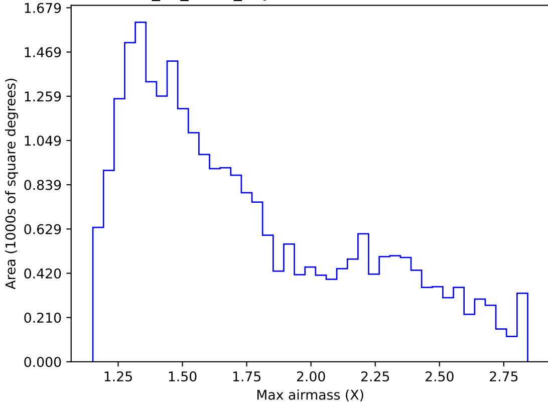
too_10_1v3.4_10yrs Yr 1 z band: Max airmass
