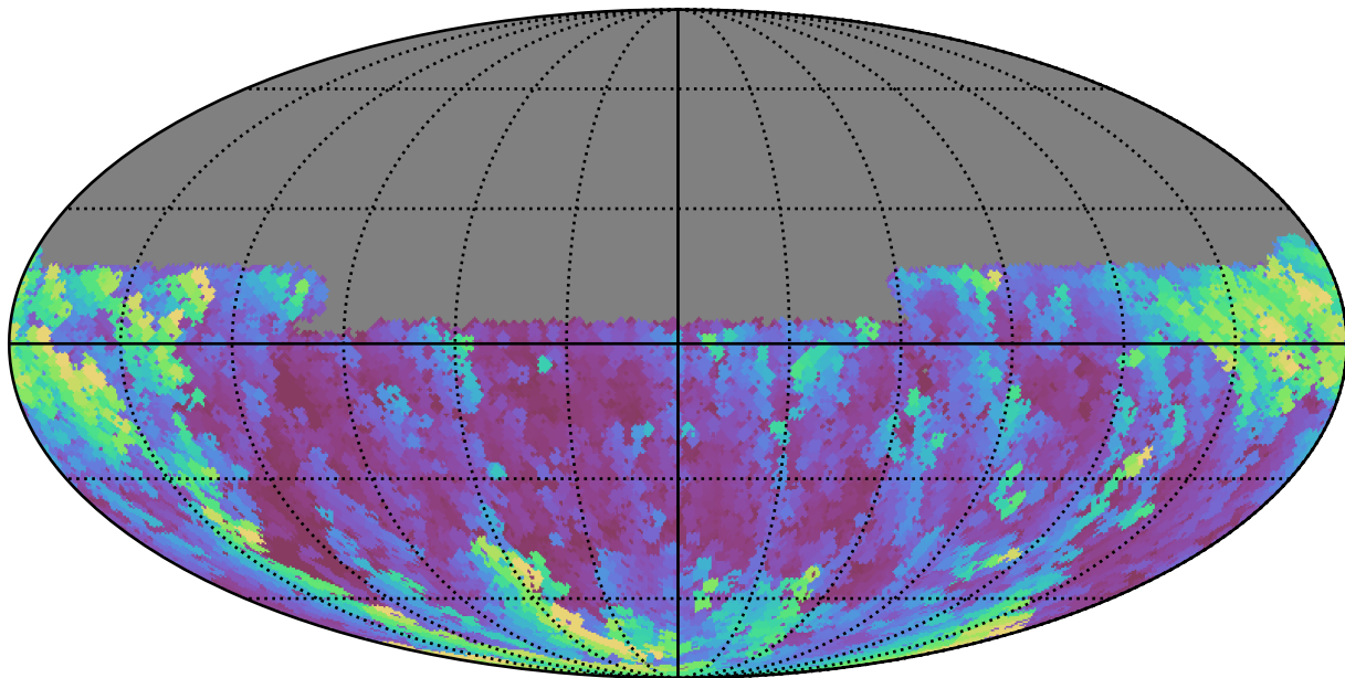
too_10_1v3.4_10yrs Yr 1 y band: Max airmass
