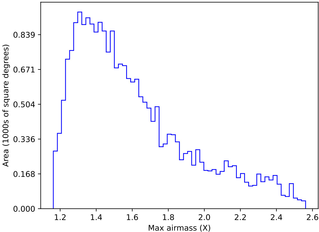
too_10_1v3.4_10yrs Yr 1 y band: Max airmass
