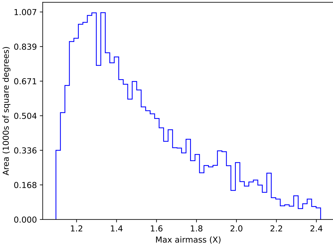
too_10_1v3.4_10yrs Yr 1 u band: Max airmass
