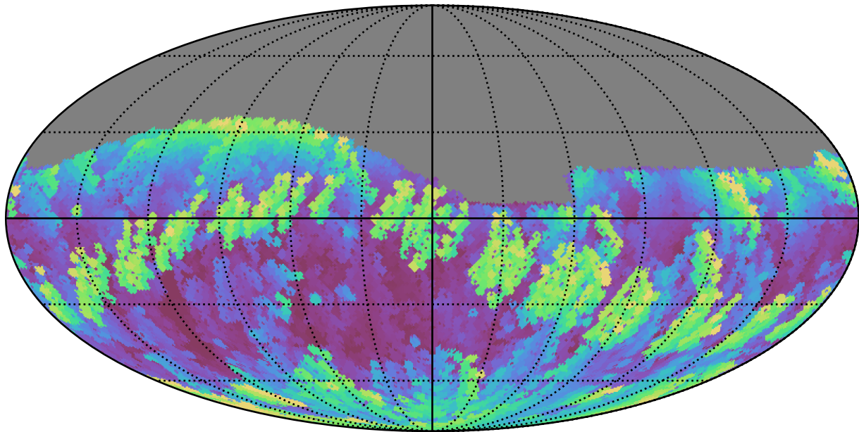
too_10_1v3.4_10yrs Yr 1 r band: Max airmass
