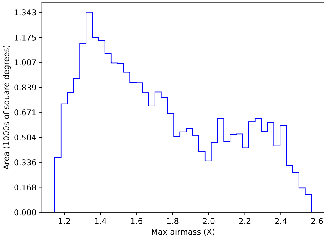
too_10_1v3.4_10yrs Yr 1 r band: Max airmass
