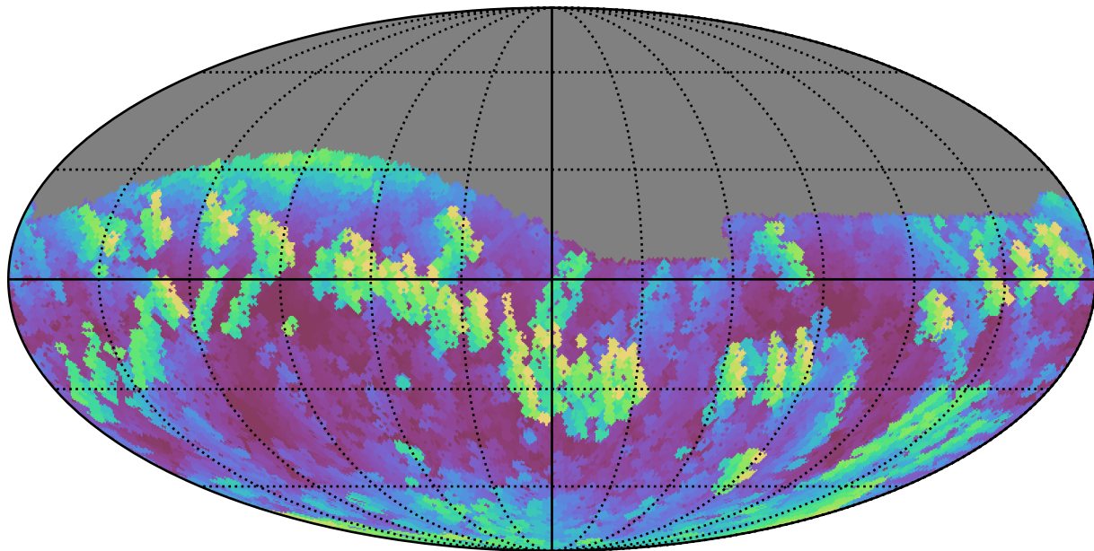
too_10_1v3.4_10yrs Yr 1 i band: Max airmass
